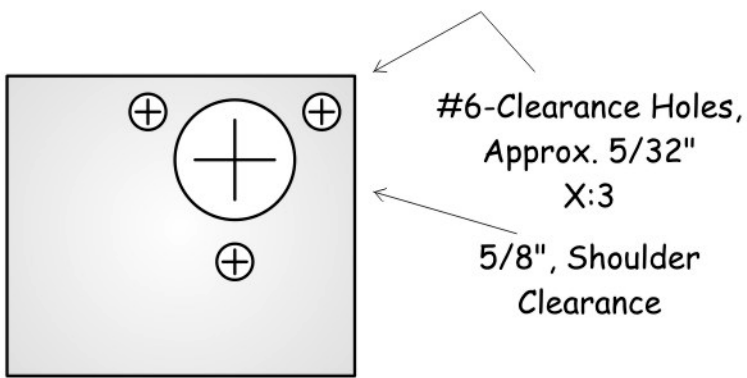
Full-Sized Drill Template
